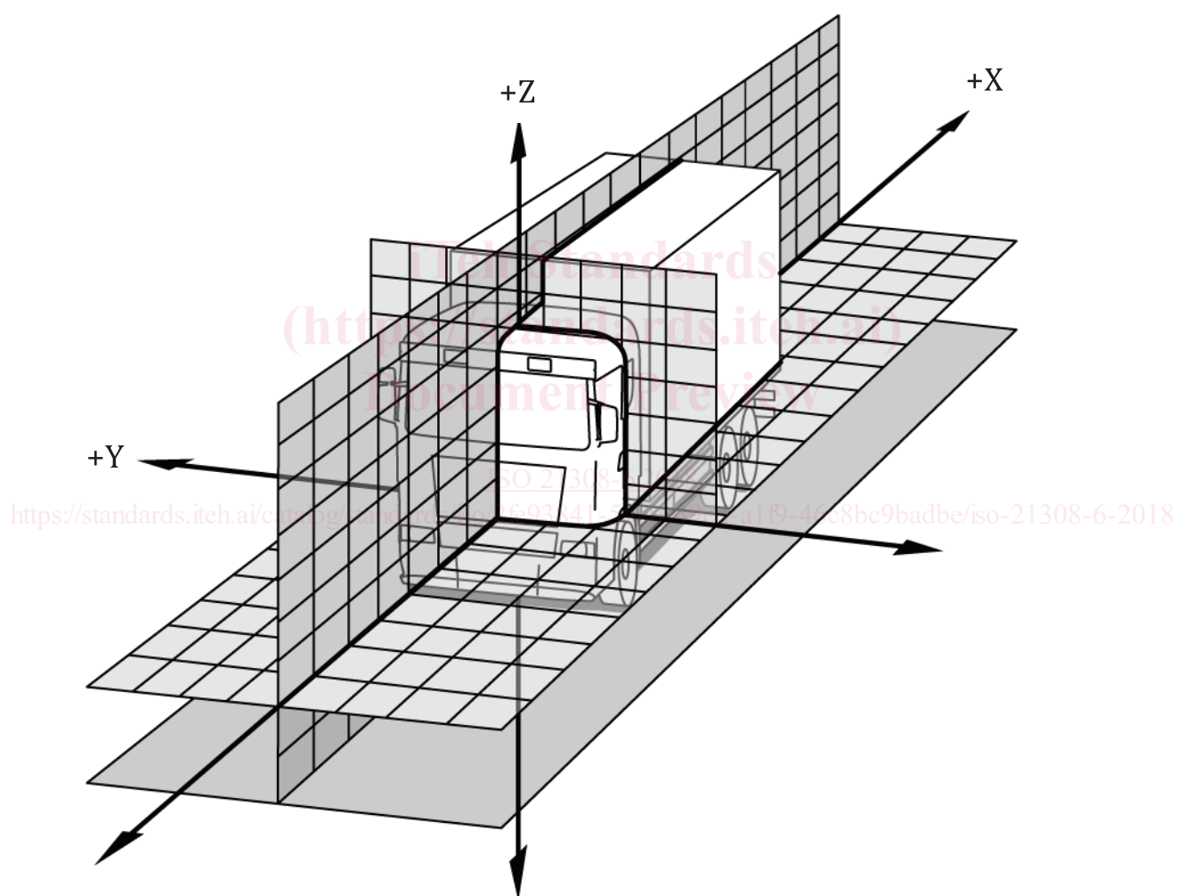
Figure 2 — Vehicle coordinate system according to ISO 4130
