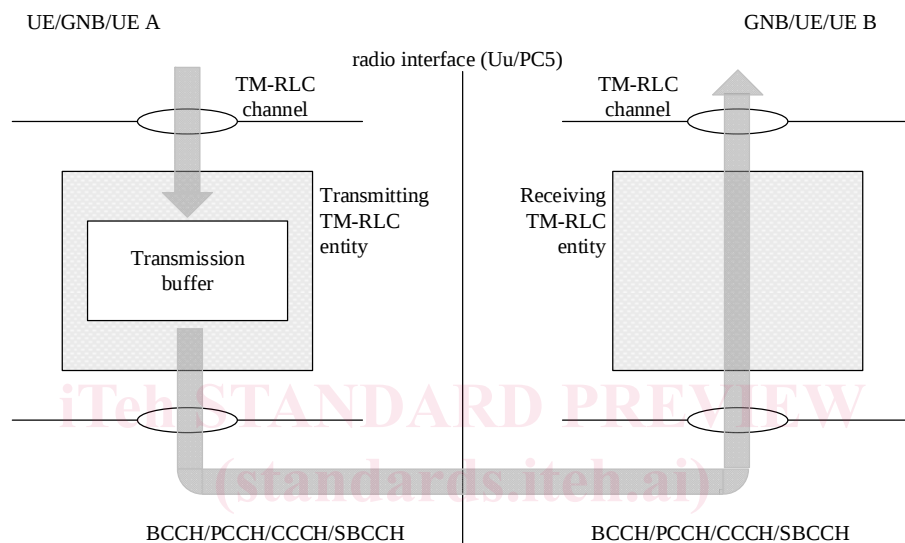
Figure 4.2.1.1-1: Model of two transparent mode peer entities
