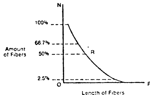
FIG. 3 Diagram Showing Digital Fibrograph Length Measurements
