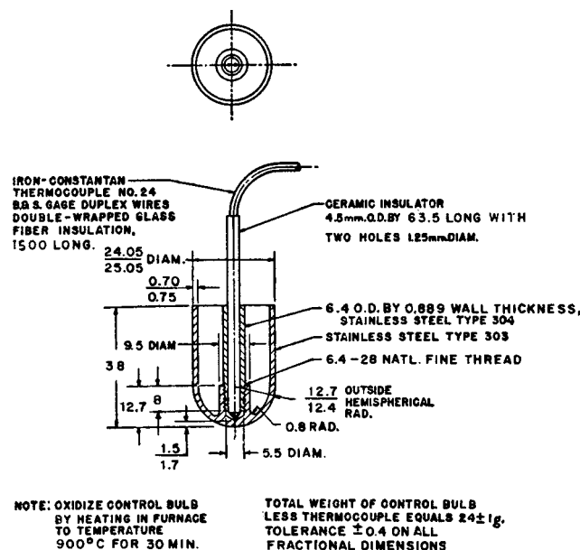
FIG. 2 Control Bulb
