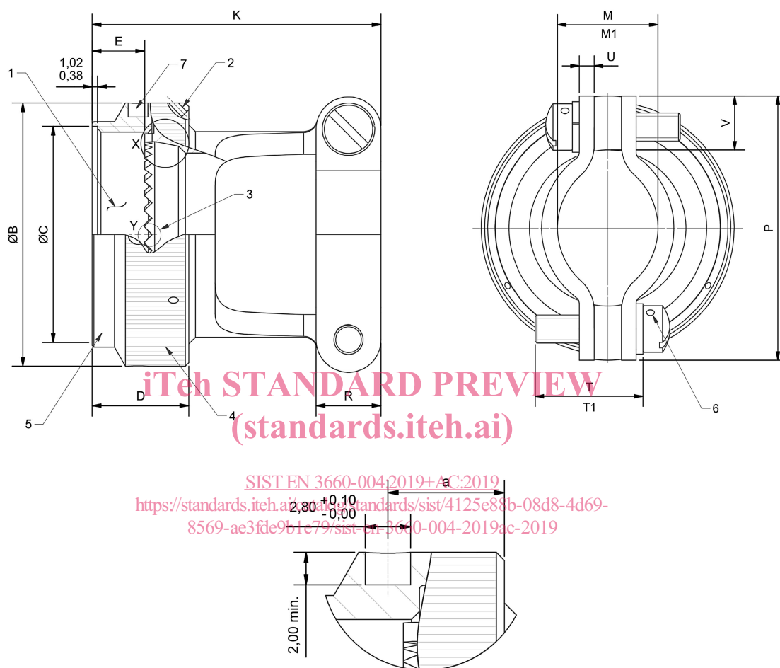
Detail Z
