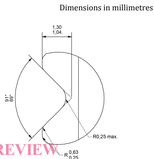
Figure 3 — Detail Y
