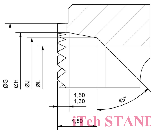
Figure 2 — Detail X
