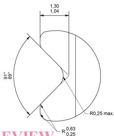
Figure 3 — Detail Y
