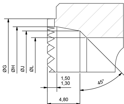
Figure 2 — Detail X
