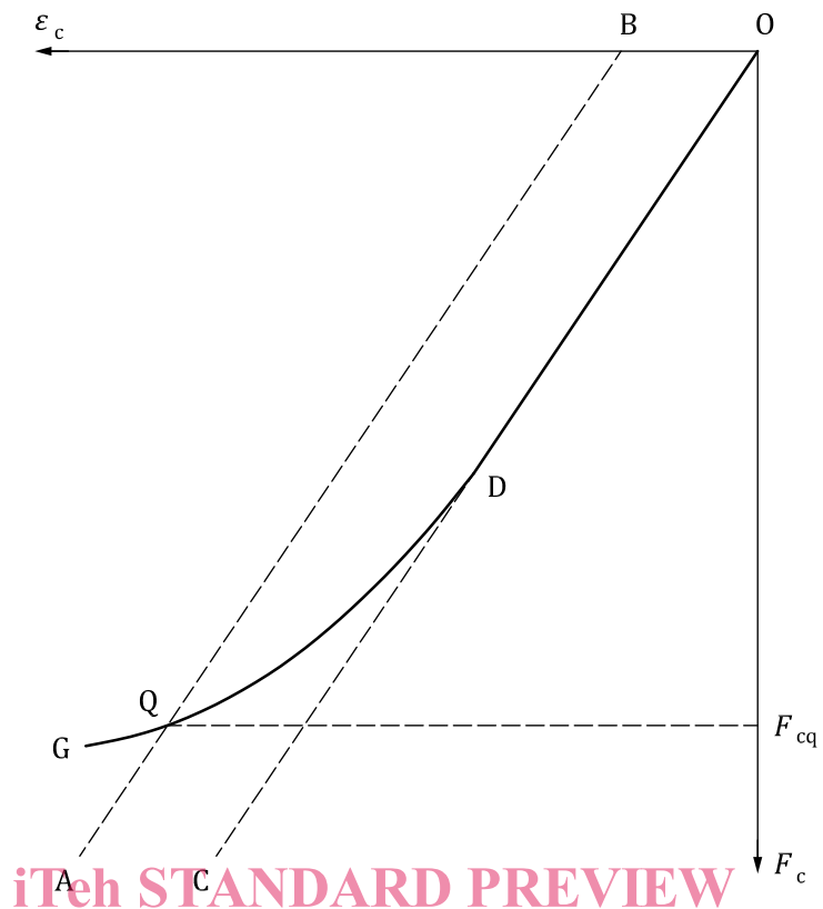
Figure 3 — Load-compression curve
