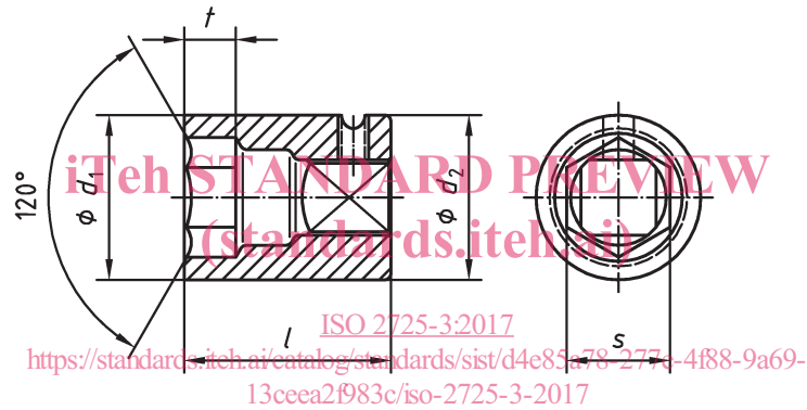
Figure 2 — Socket shown with type J square conforming to ISO 1174-2
