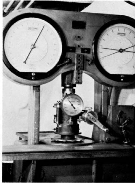
FIG. 3 Hveem Stabilometer Placed in the Testing Machine
