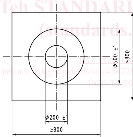
Figure 1 — Baseplate
