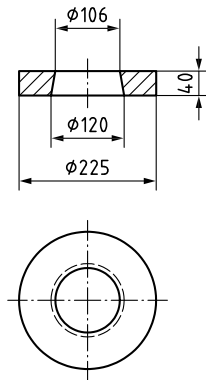
Figure 2 — Example of dimensions of a steelwighted collar
