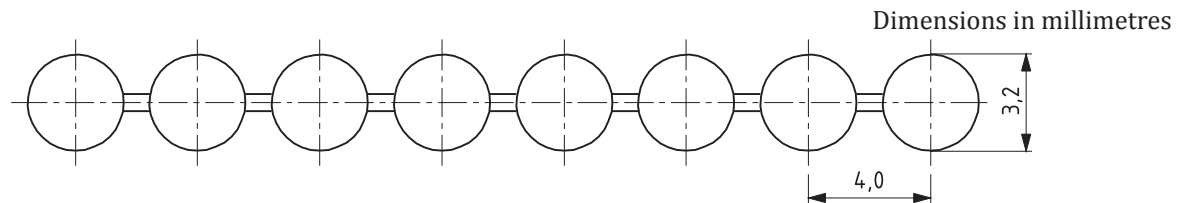
Figure 4 — Ball chain
