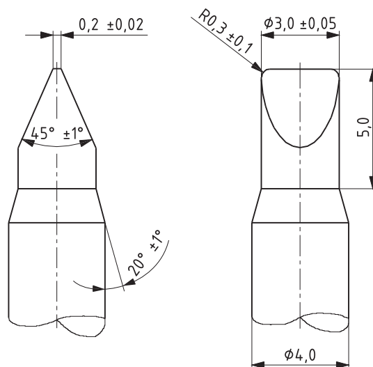
Figure 7 — Test teeth
