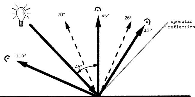
FIG. 2 Diagram of Aspecular Angles
