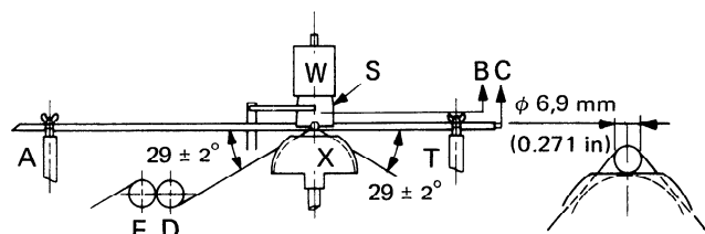
FIGURE 3 — Details of the abrasive mechanism
