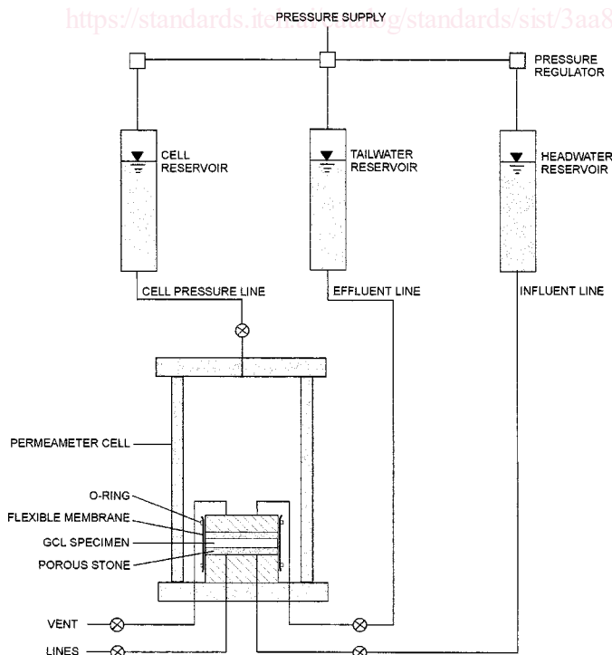
FIG. 1 Permeameter Cell and Test Setup
