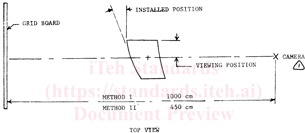
FIG. 2 Example of Installed Angle
