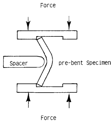
FIG. 4.7 Schematic Fixture for Completing the Guided-Bend Test Started as Shown in Fig. 3
