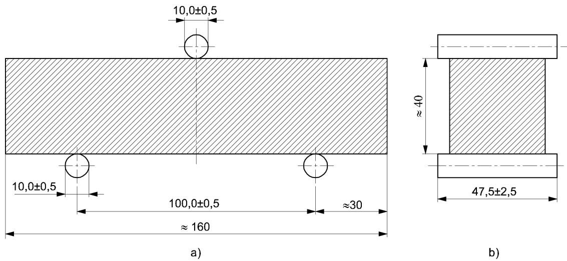
Figure 1 — Arrangement of loading for determination of flexural strength
