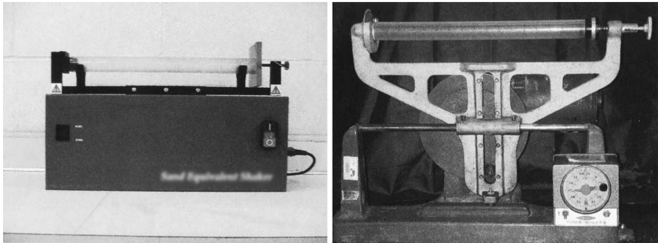
FIG. 2 Mechanized Shakers
