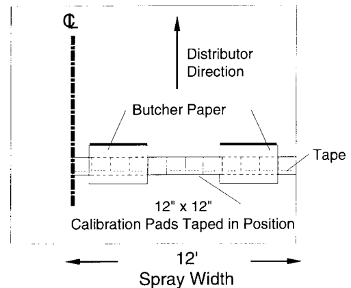
FIG. 2 Position of Calibration Pad Assemblies for Transverse Rate Determination
