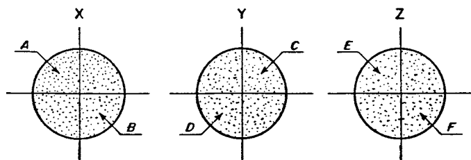
FIG. 2 Quartering Samples
