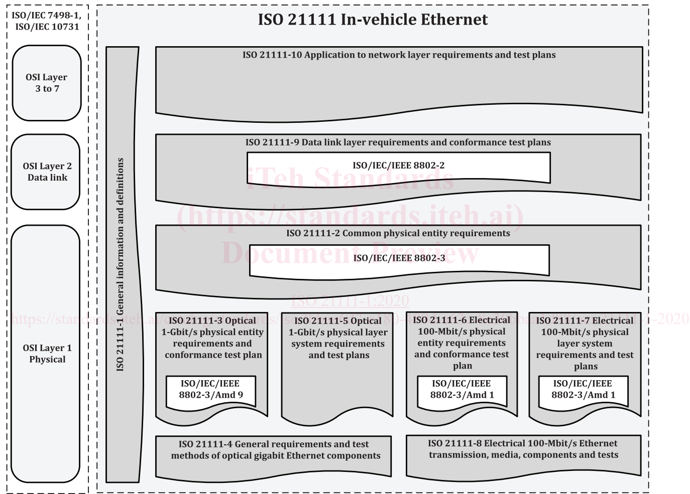
Figure 1 — In-vehicle Ethernet document reference according to OSI model
