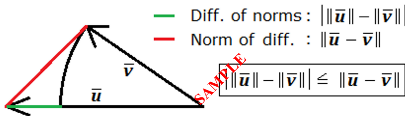
Figure 1 — Triangle Inequality
