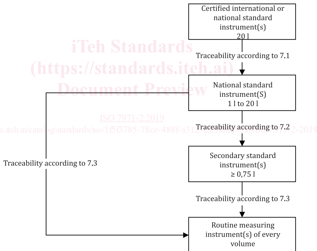
Figure 1 — Principle of traceability of instruments through reference to standard instruments
