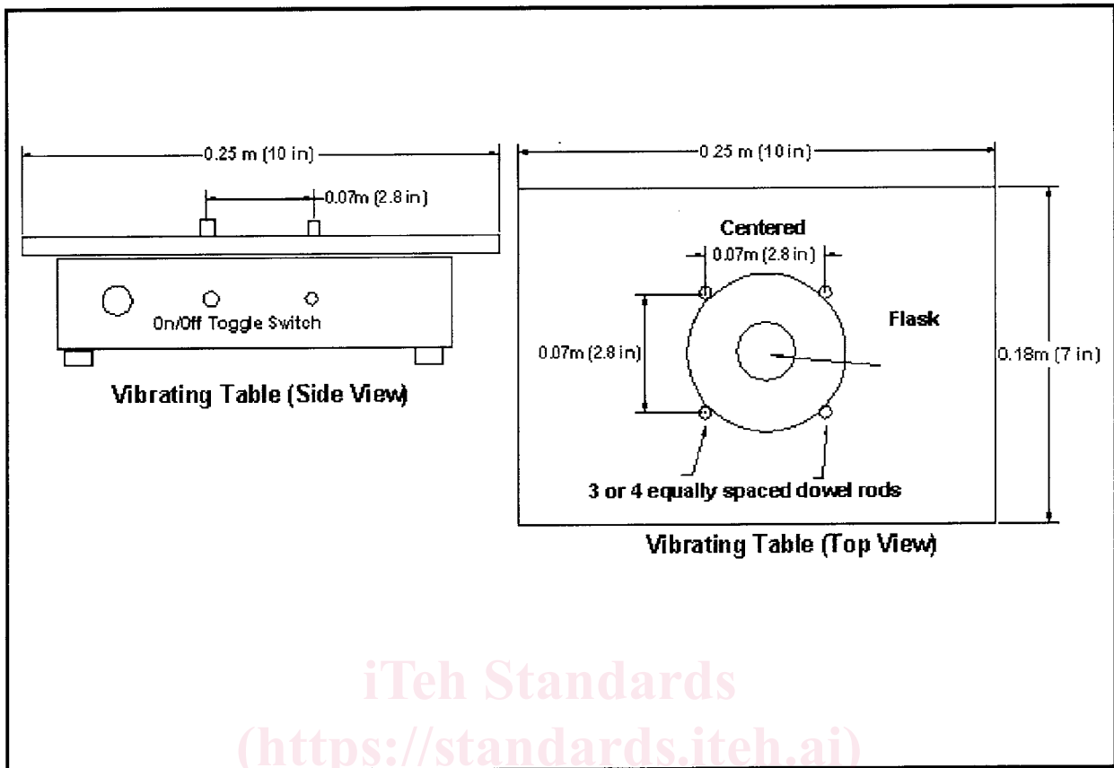
FIG. 1 Vibrating Table
