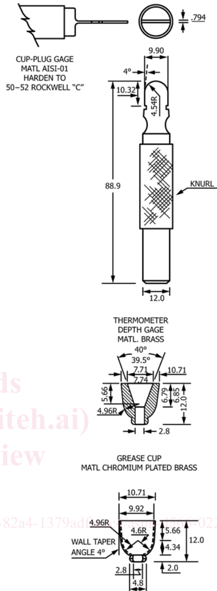
FIG. 1 Plug Gage, Depth Gage, and Grease Cup
