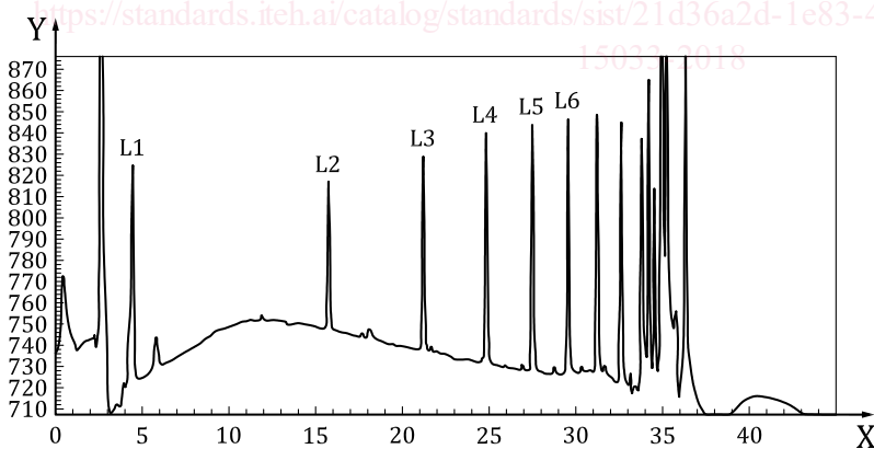
Figure 1 — Determination of the cyclic oligomers of caprolactam — Method A, example — UV chromatogram
