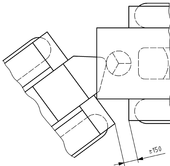
Figure 1 — Minimum clearance of lower limbs at access to the operator's station on machines with articulated steering
