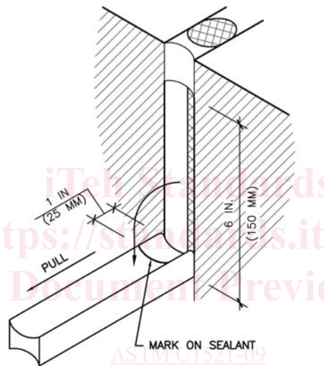
MARK CUT PORTION OF SEALANT 1 IN. (25 MM) FROM ADHESIVE BOND. PULL TAIL.
