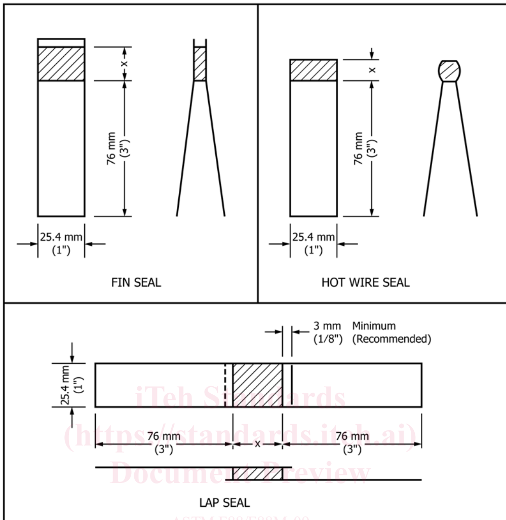
NOTE 1—Seal dimension marked X varies with sealer configuration.
