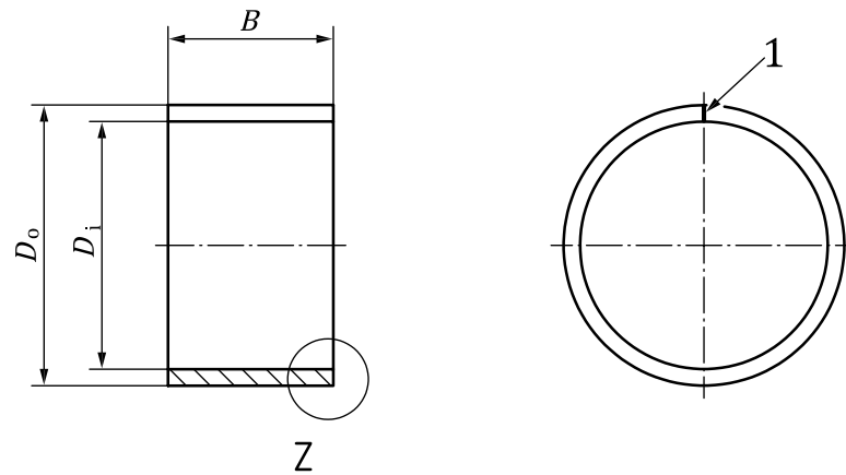
a) Type C cylindrical bush
