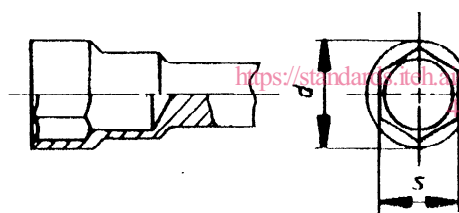
Figure 1 — Socket wrench, forged type
