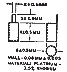
FIG. 11 Weighing Cup
