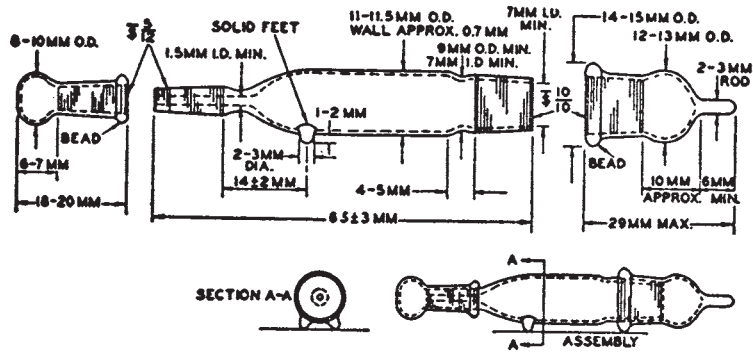
FIG. 7 Weighing Bottle, Pig-Type, with Two Caps
