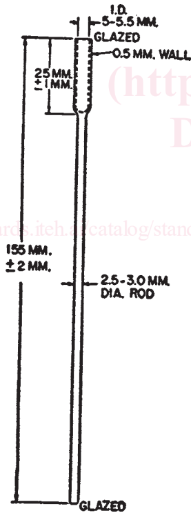
FIG. 12 Weighing Tube
