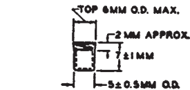
FIG. 4 Weighing Bottle
