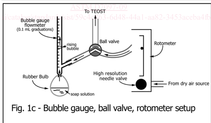
FIG. 1 Bubble Gauge
