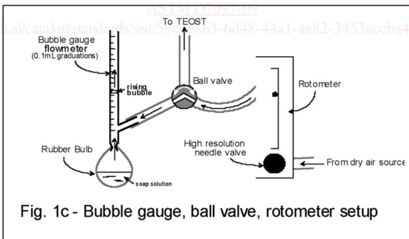
FIG. 1 Bubble Gauge
