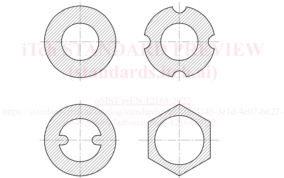
Figure 1 — Examples of hollow rod cross-sections
