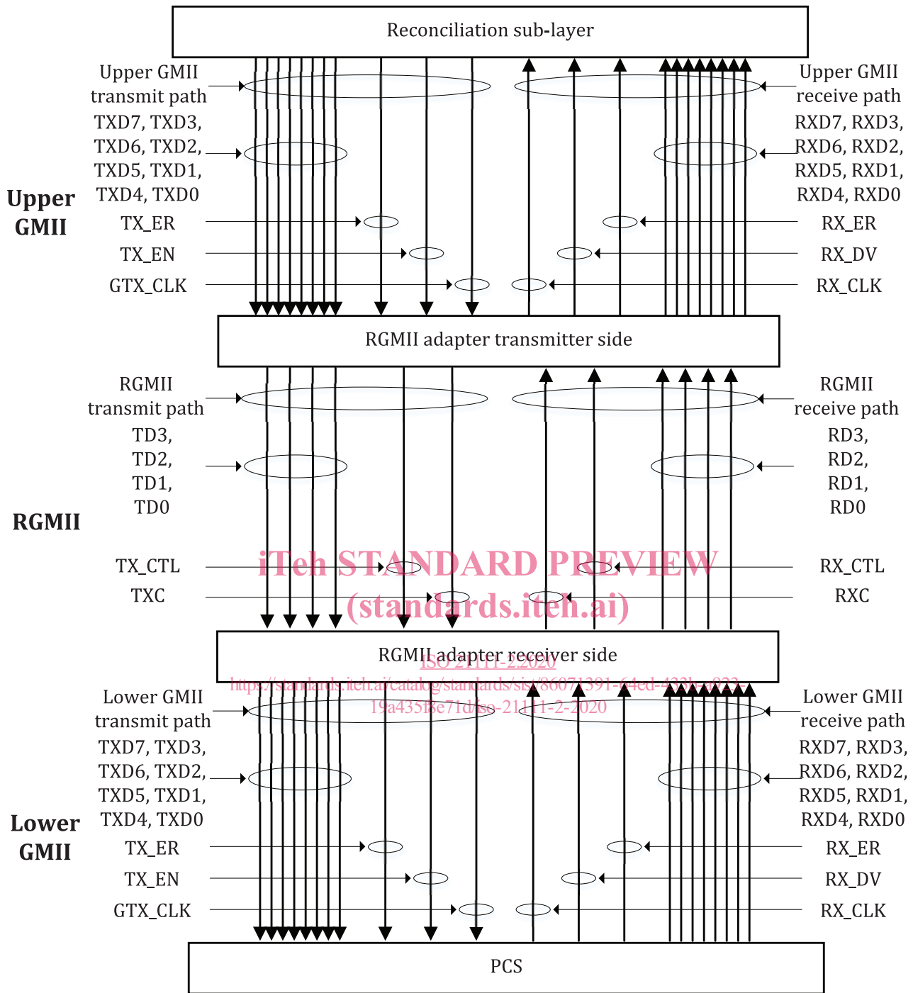
Figure 2 — RGMII architecture
