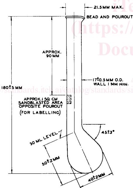
FIG. 3 30-mL (Soltys) Kjeldahl Flask
