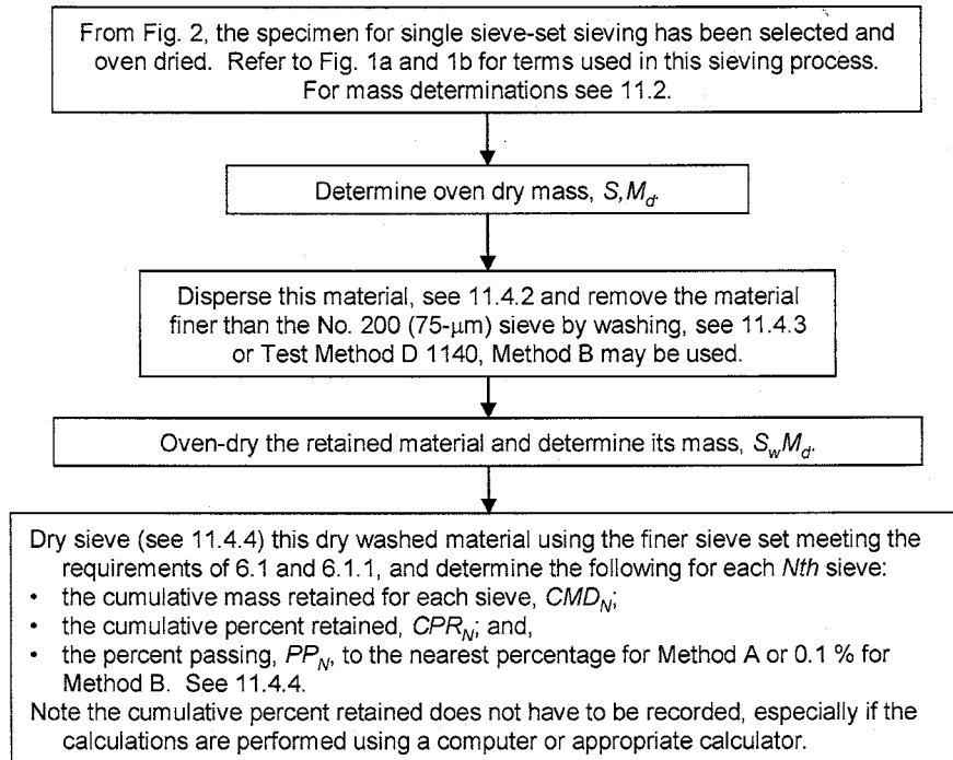
FIG. 3 Flowchart for Single Sieve-Set Sieving
