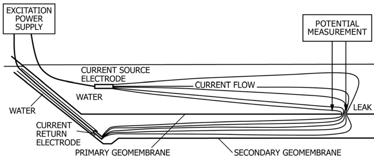
FIG. 1 Diagram of the Electrical Leak Location Method for Surveys with Water Covering the Geomembrane
