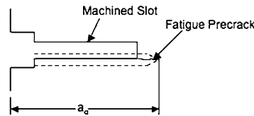
Notch and Precrack Configurations
