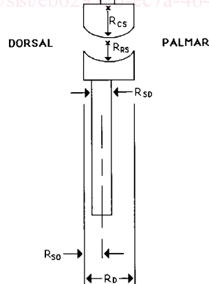
FIG. 2 Dimensions of Wrist Joint Replacements (Sagittal Plane)
