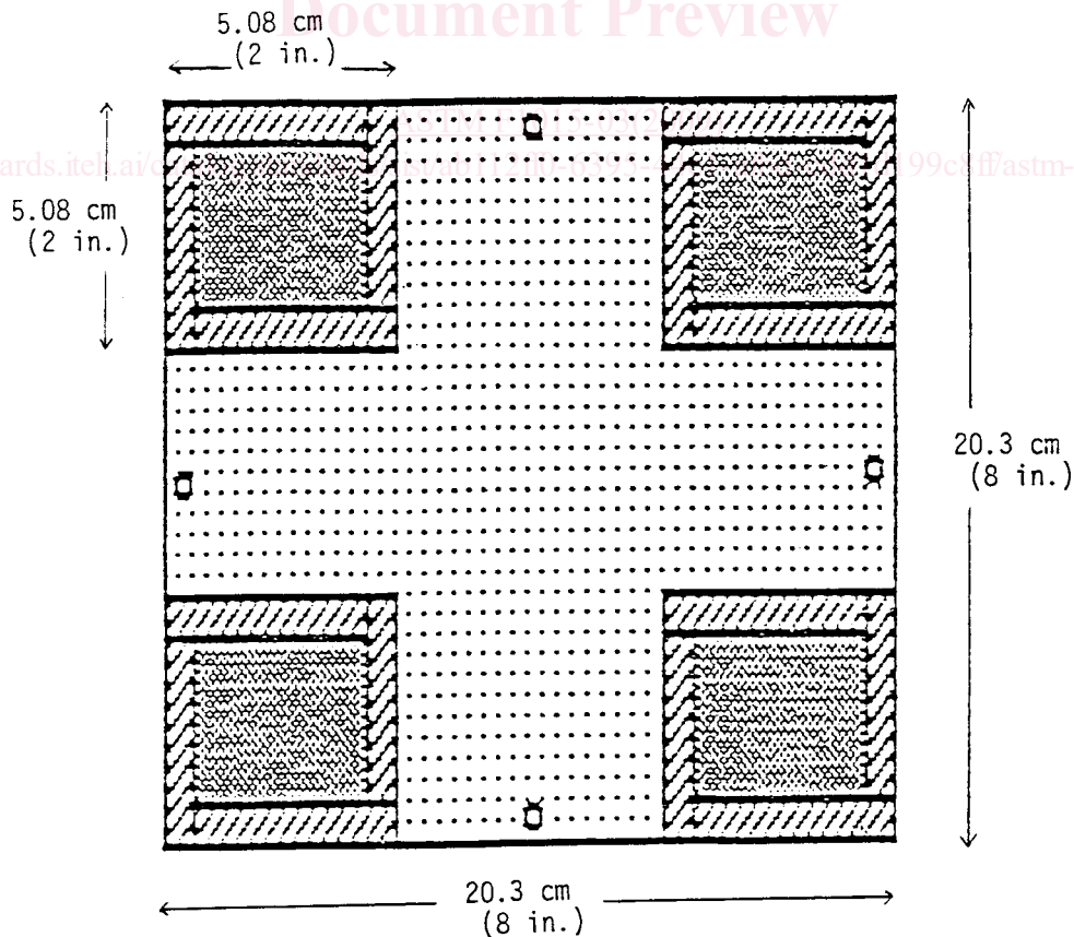
FIG. 1 Test Fixture
