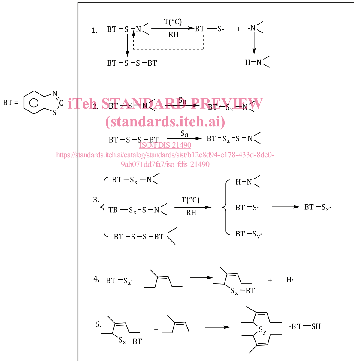
Figure A — Reaction of sulfenamides during the curing of a rubber compound
