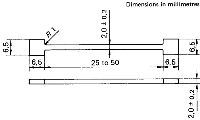
Figure – Test piece with enlarged ends
