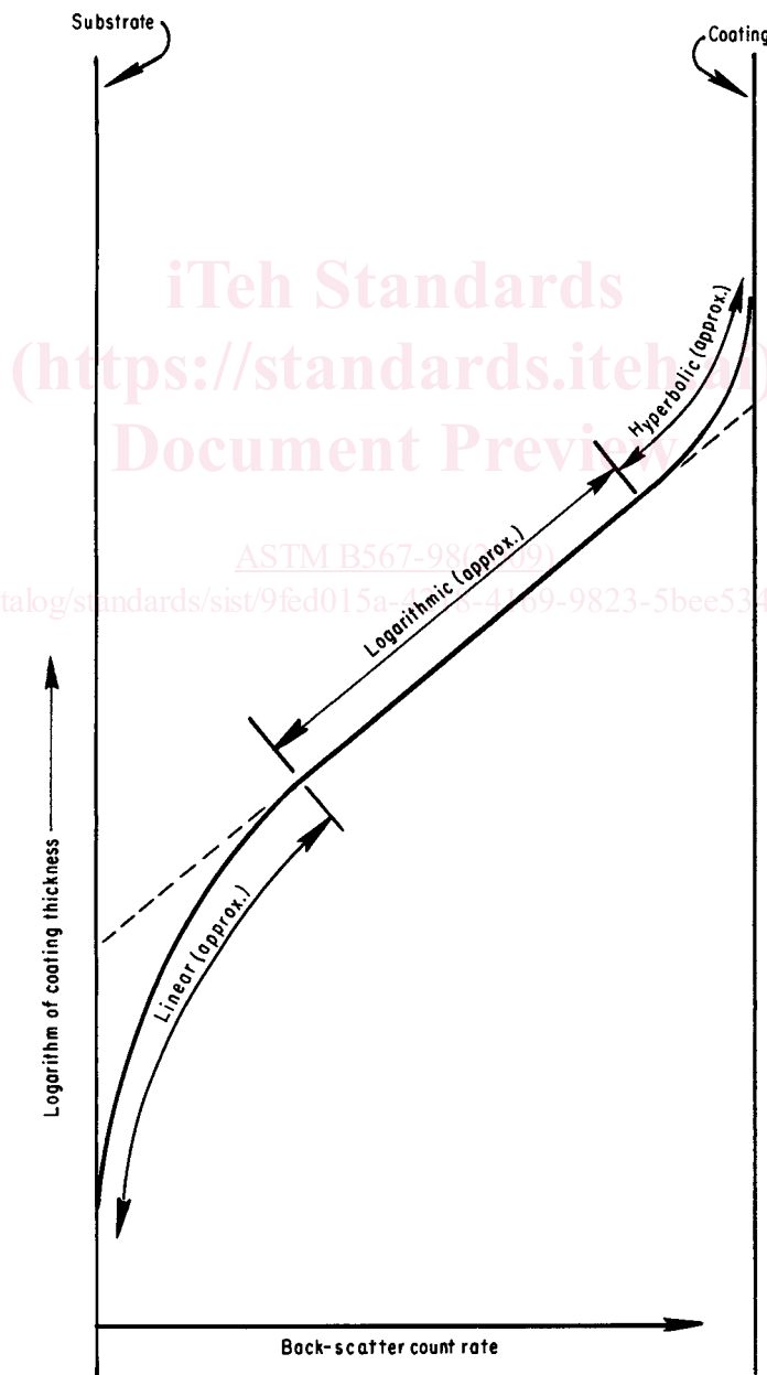
FIG. 1 Normalized Backscatter
