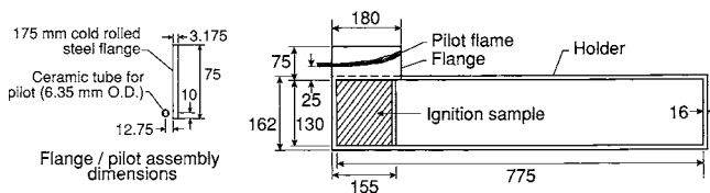
FIG. 3 Pilot Configuration for Ignition Test
