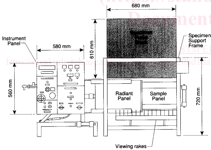
FIG. 5 Test Apparatus Main Frame, Front View
