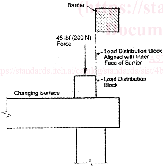
FIG. 3 Stability Test
