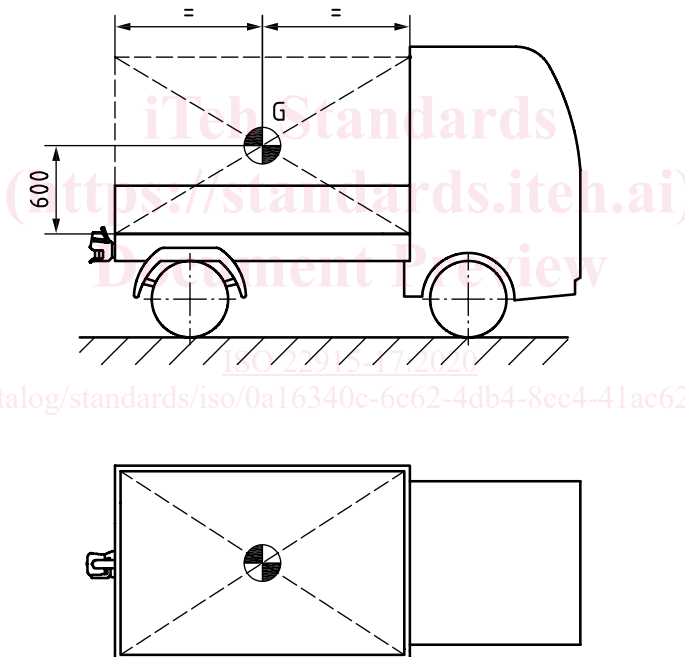
Figure 1 — Indication of the minimum height of the centre of gravity, G
