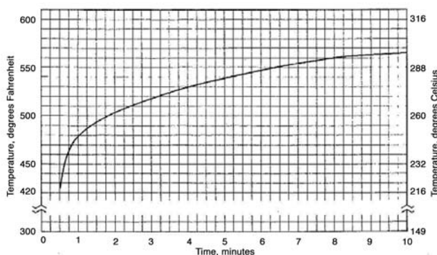
FIG. 6 Representative Time-Temperature Curve for Preheat Temperatures
