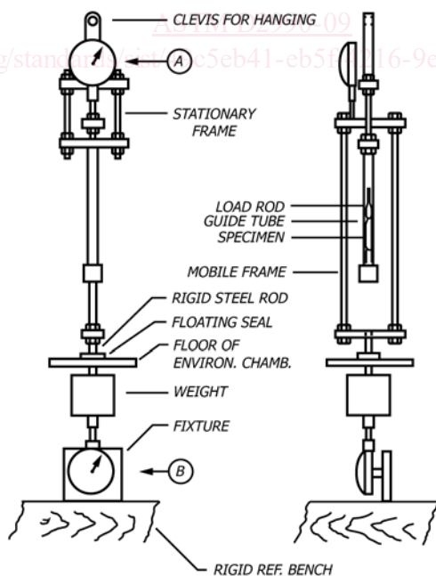
(A) LOCATION OF DIAL INDICATOR WHEN NOT USED IN ENVIRONMENTAL CHAM. (B) LOCATION OF DIAL INDICATOR WHEN USED IN ENVIRON. CHAMBER.
