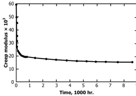
FIG. X2.3 Creep Modulus versus Time
